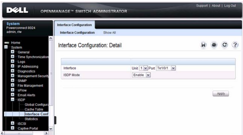
Figure 23-3. ISDP Interface Configuration
