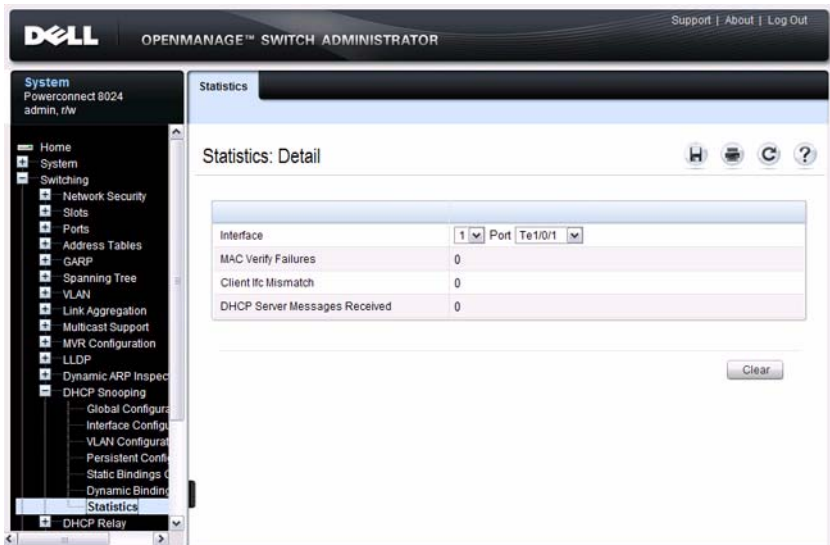
Figure 26-11. DHCP Snooping Statistics
