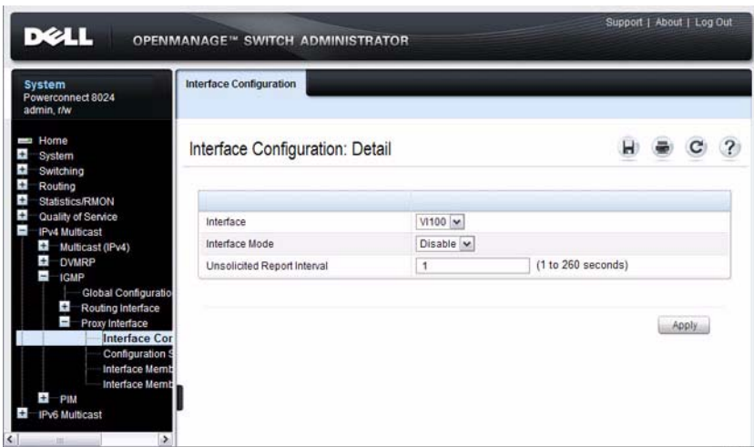
Figure 42-14. IGMP Proxy Interface Configuration
