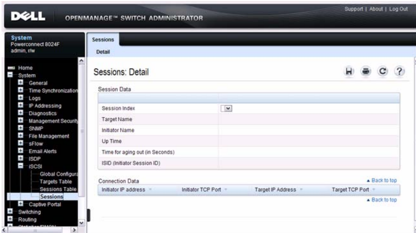
Figure 16-5. iSCSI Sessions Detail
