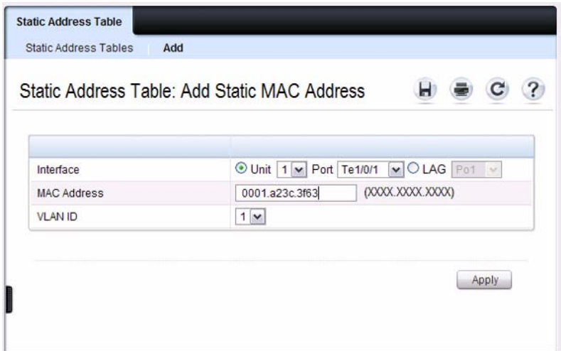
Figure 29-2. Adding Static MAC Address
