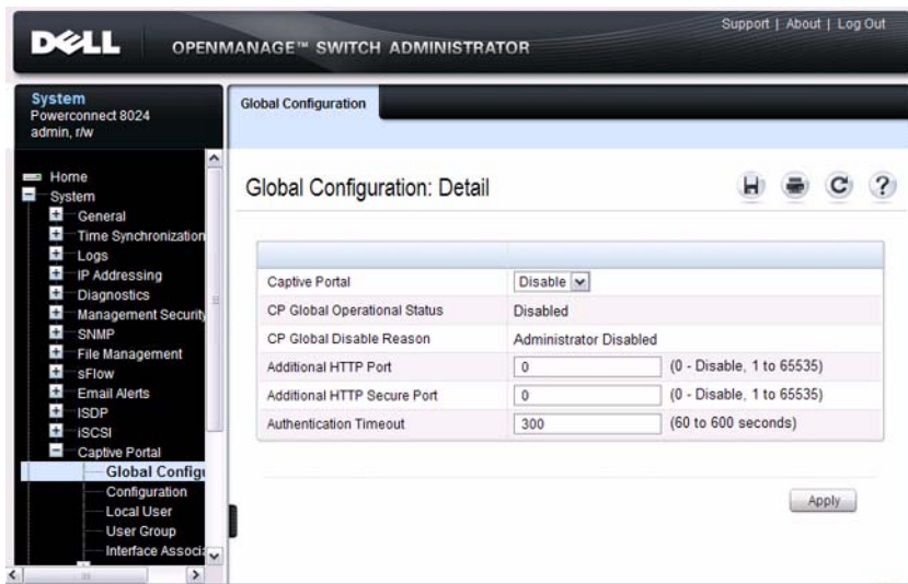
Figure 17-4. Captive Portal Global Configuration
