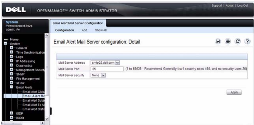
Figure 10-15. Email Alert Mail Server Configuration
