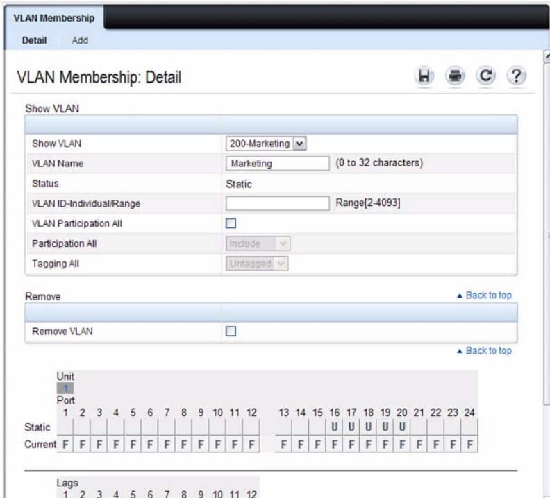
Figure 21-27. VLAN Membership - VLAN 200
