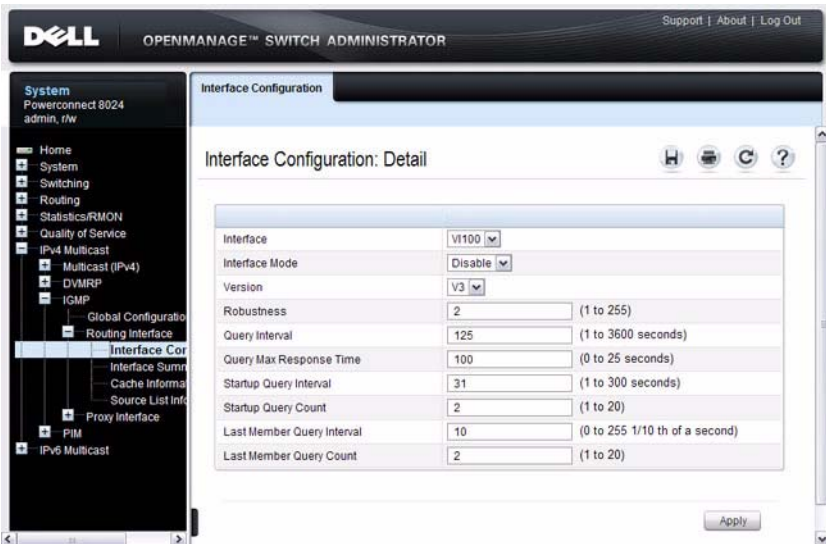
Figure 42-10. IGMP Interface Configuration
