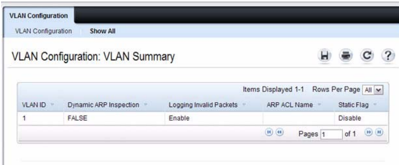
Figure 26-19. Dynamic ARP Inspection VLAN Configuration Summary
