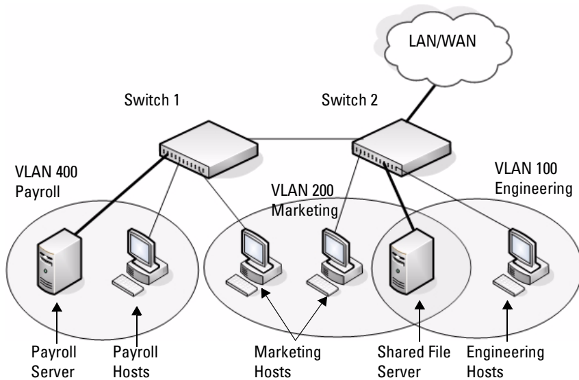
Figure 21-25. Network Topology for Port-Based VLAN Configuration
